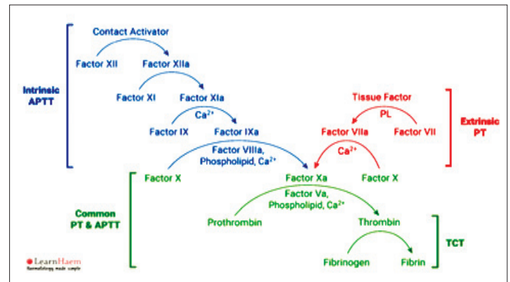
Figure 1: Coagulation Cascade
